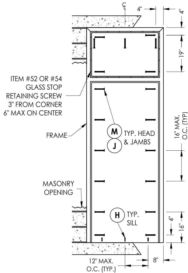
FRAME ANCHORING
