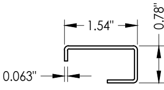
86 GLASS STOP
