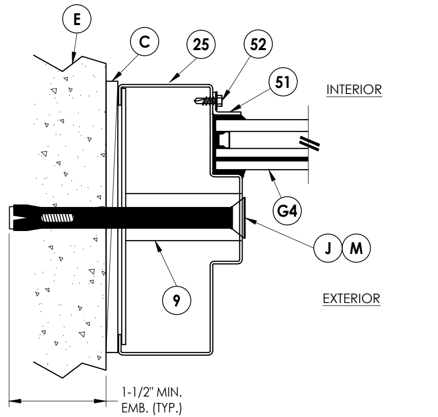
4 HORIZONTAL CROSS SECTION 3 Optional glazing
