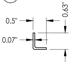
51 FIXED GLASS STOP
