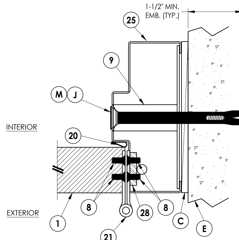
2 HORIZONTAL CROSS SECTION
